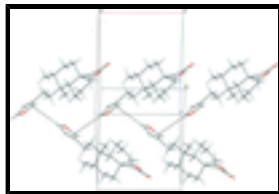
Fig. 2. Unit cell packing of the title compound showing C—H... \pi interactions as dashed lines.
