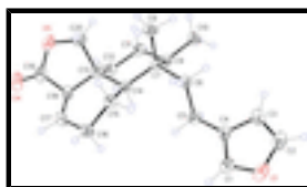
Fig. 1. Molecular structure of the title molecule with atom labels drawn with displacement ellipsoids at 50% probability level.
